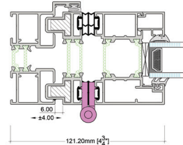
121.20mm [4 3/4"]
